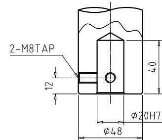
SHANK HOLE
